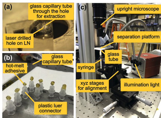
Fig. 8 (a) An 80 \mu\text{m} outer diameter glass capillary tube is inserted into a 100 \mu\text{m} diameter hole in LN substrate for the extraction platform. (b) A luer lock connector is attached to the glass capillary tube using hot-melt adhesive to facilitate syringe attachment. (c) Image of the extraction platform, including lab-based components for system alignment.
