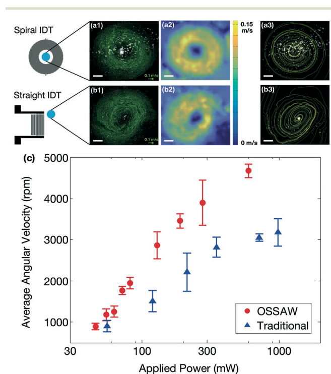
Fig. 3 A comparison between (a) OSSAW and (b) traditional offset droplet spinning using a straight IDT configuration may be made from (a1 and b1) vector velocity, (a2 and b2) velocity magnitude, and (a3 and b3) particle streamlines for a 1.5 \mu\text{L} DI water droplet. Average eccentricities of 0.28 and 0.81, respectively, were computed from the streamlines of (a3) the OSSAW and (b3) traditional straight IDT devices. These streamlines were calculated using PIVlab, suggesting an improved axisymmetric droplet spinning via OSSAW. (c) The OSSAW also produces a greater average angular velocity (rpm) for a given applied power. The maximum possible rotation speed from the traditional design at any power is 3180 rpm; the droplet is ejected from the surface at greater input powers. However, with OSSAW, a speed of 4670 rpm may be achieved, at which point atomization begins to appear. The error bars represent the standard deviation ( n = 5 for each data point).
